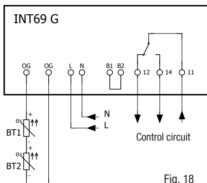
Fig. 18 Terminal box
